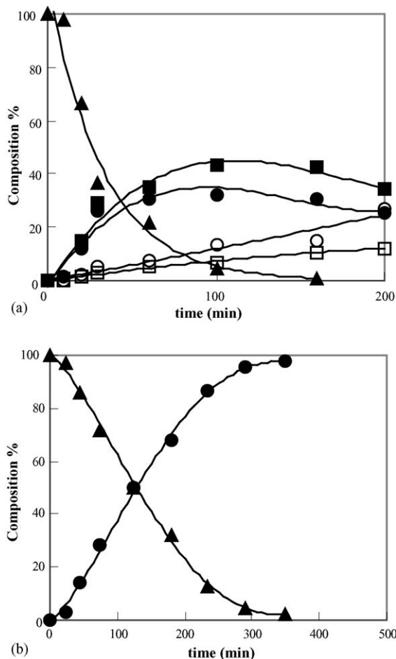
Fig. 1. Product distribution (mol%) during the course of acetophenone hydrogenation (353 K, 1 MPa H 2 , 0.25 g catalyst): (a) Pt/SiO 2 catalyst; (b) PtSn-OM catalyst. (▲) Acetophenone, (●) 1 , (■) 2 , (○) 3 , (□) ethylbenzene and ethylcyclohexane).
